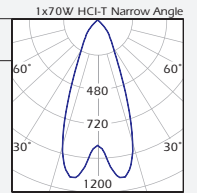
cd/km — C0-C180 — C90-C270 1x70W HCl-T Wide Angle
